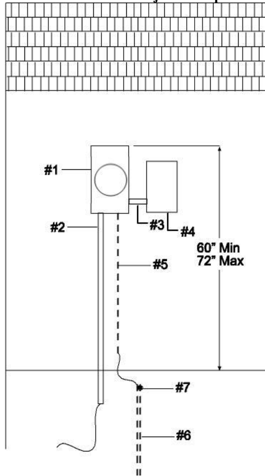
200 Amp UnderGround Meter Loop with Galvanized Nipple
