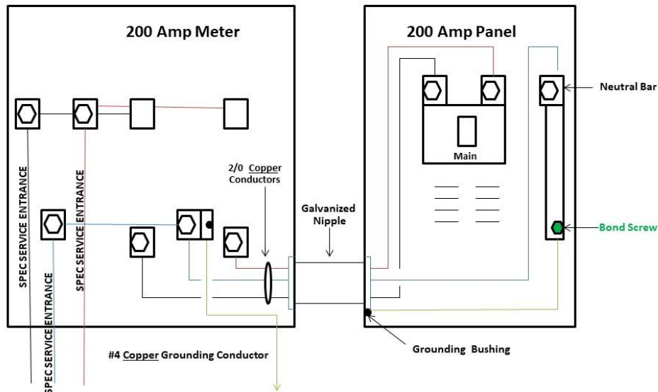
200 Amp UnderGround Meter Loop with Galvanized Nipple
