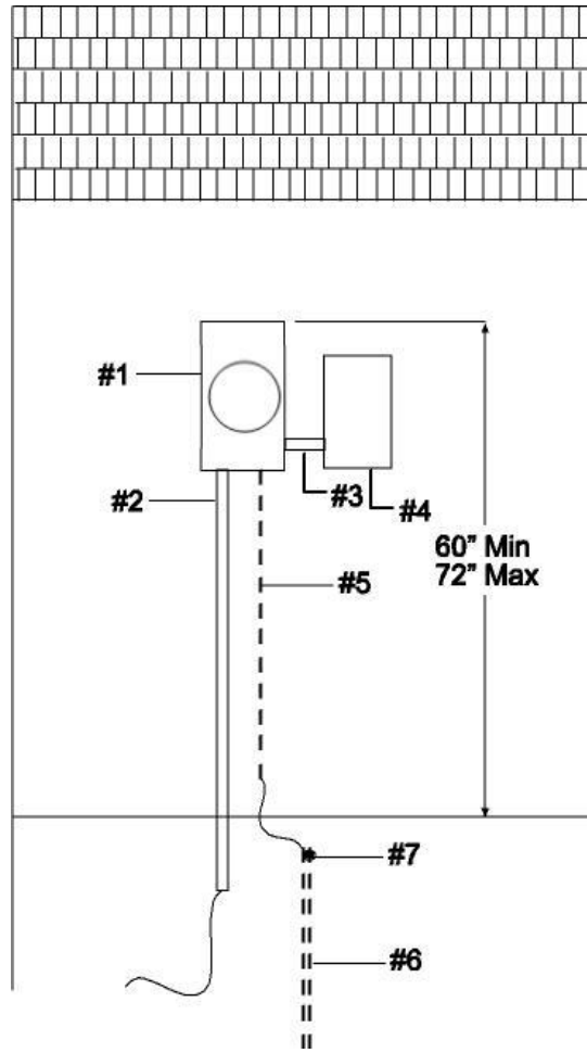
200 Amp UnderGround Meter Loop with Galvanized Nipple
