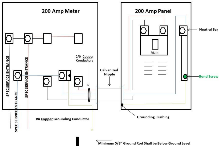
200 Amp UnderGround Meter Loop with Galvanized Nipple
